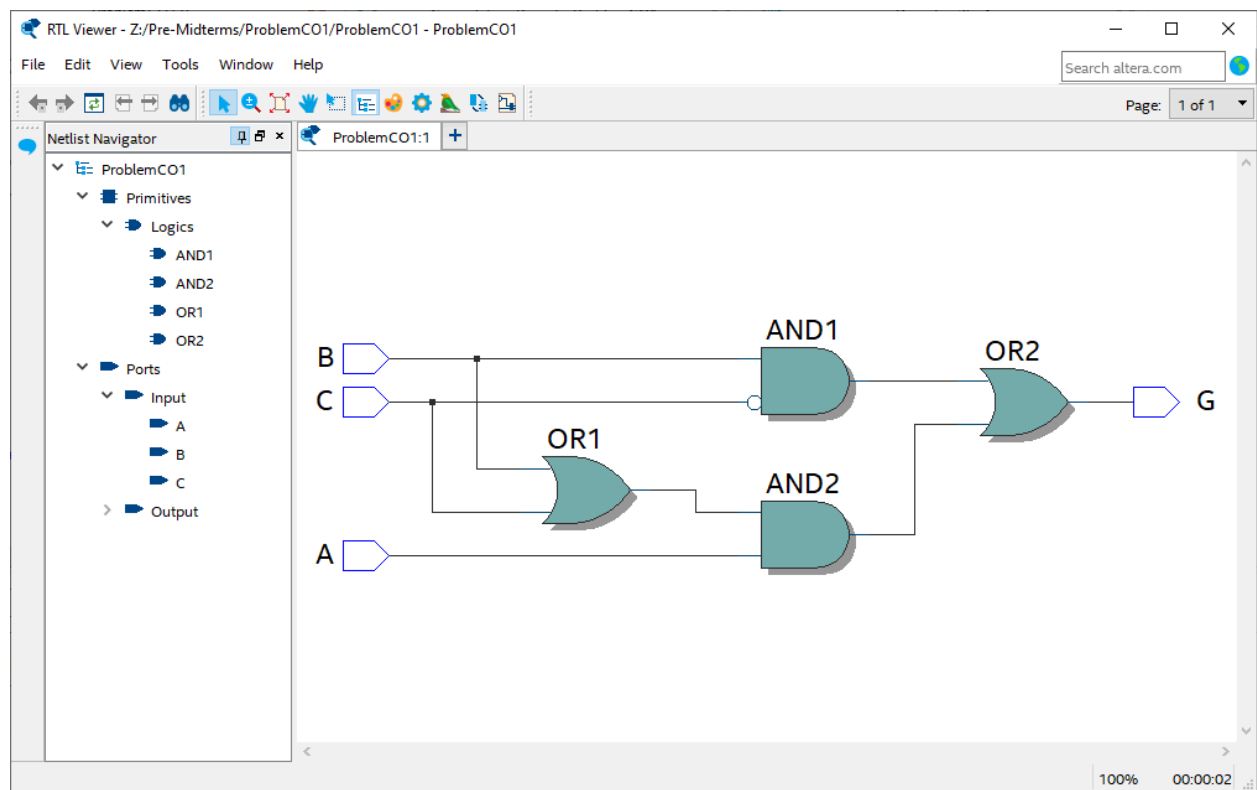
Figure 3. RTL Schematic Diagram of ProblemCO1.v
